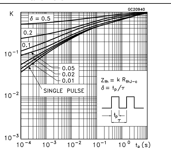
Figure 3. Thermal impedance for TO-220FP and TO-3PF
