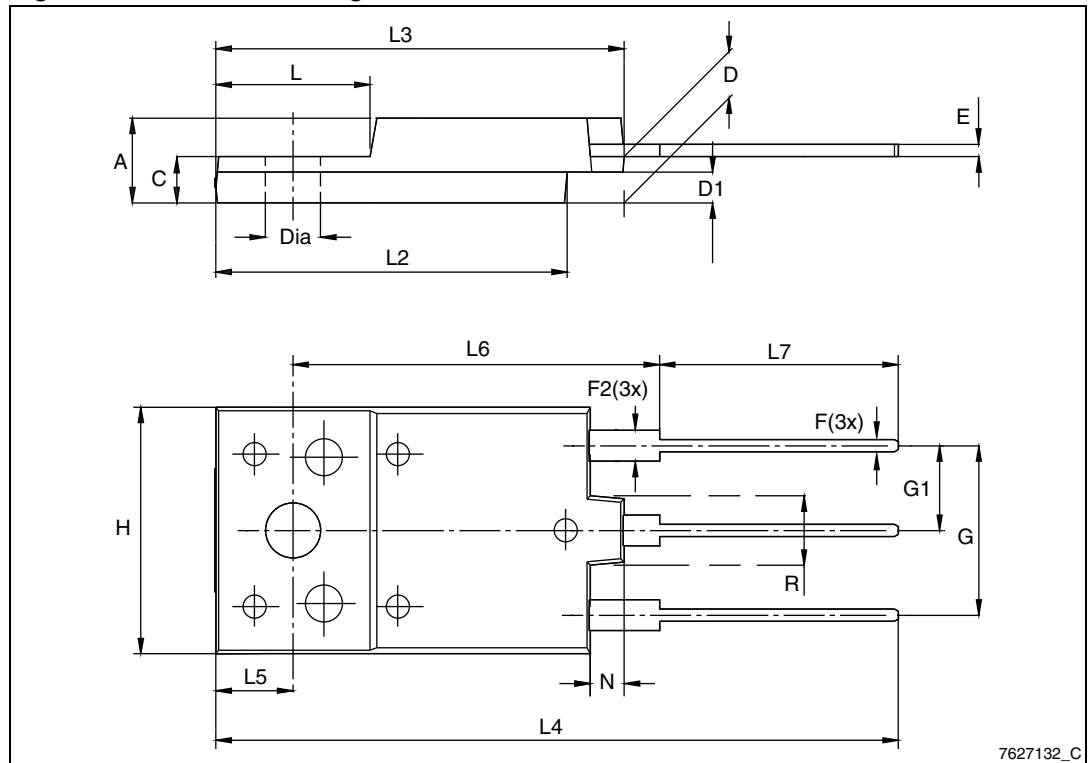
Figure 24. TO-3PF drawing
